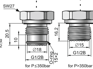
CG1/2 type G1/2" with flush diaphragm
