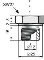
GP type G1/2", Ø12 hole P type M20x1.5, Ø12 hole
