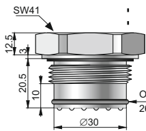
G1/2 type G1/2", Ø4 hole M type M20x1.5, Ø4 hole
