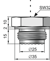
CM30x2 type M30x2 with flush diaphragm
