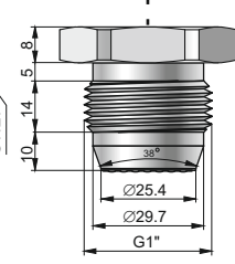
CG1-S38 type G1" with flush diaphragm
